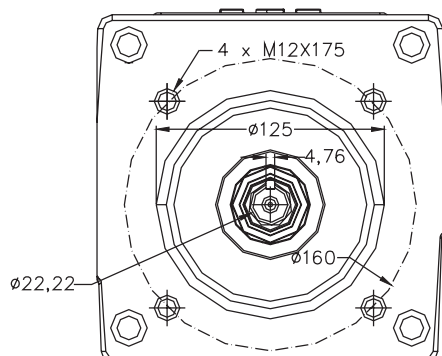
Electrical motor coupling bell according to ISO 4
